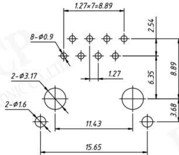
PCB Layout
